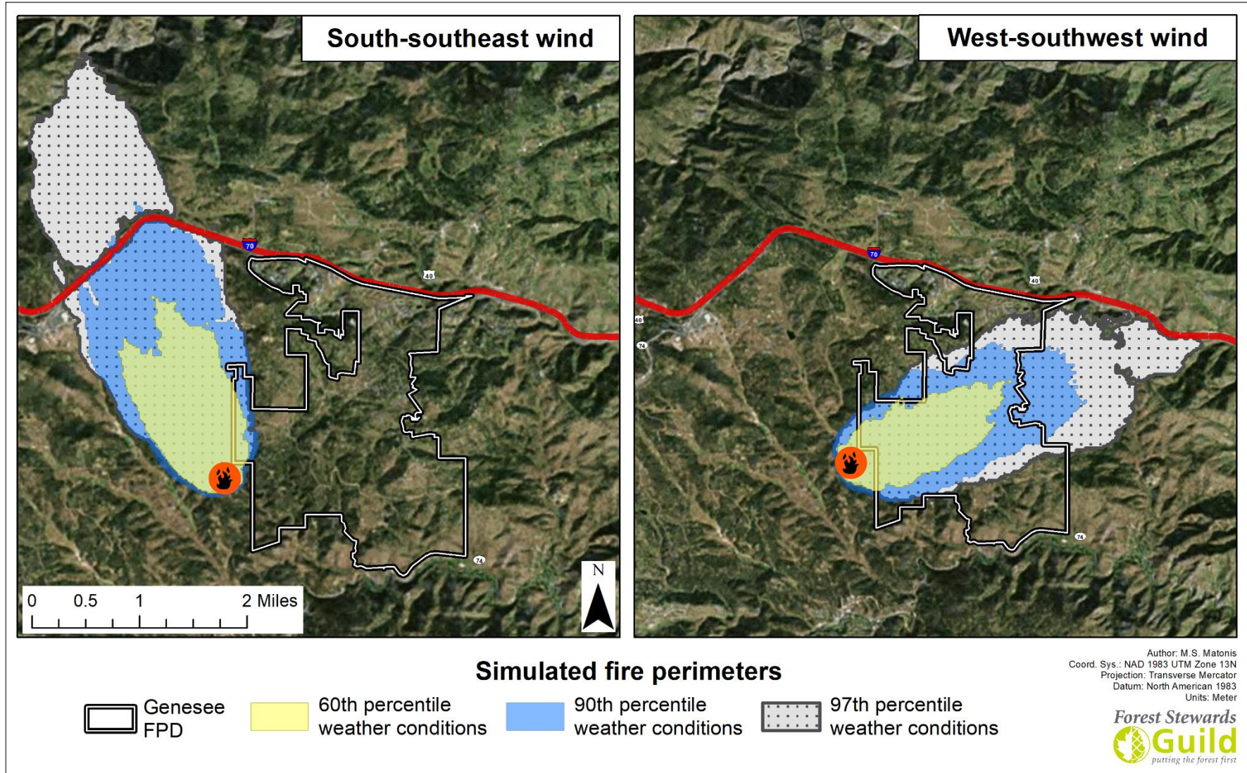
Figure 3b.6. Simulated fire perimeters after 4-hours of fire growth without suppression activities originating from an ignition to the west of the GFPD. We modeled fire growth using FlamMap’s minimum travel time algorithm and 60 th , 90 th , and 97 th percentile fire weather conditions under prevailing winds out of the south-southeast and west-southwest.
